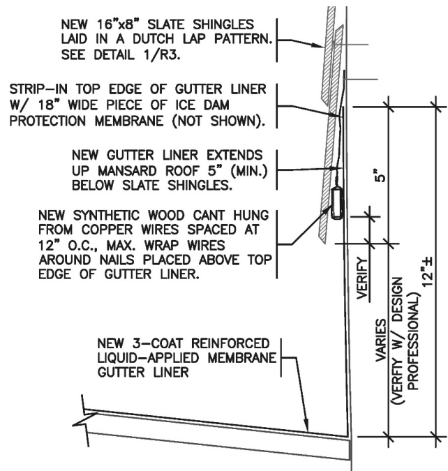
Figure 7: Section showing cant and first course of slate above a built-in gutter.
