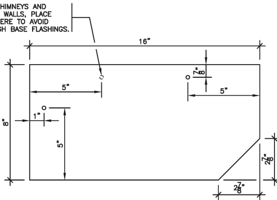
NEW SLATE SHINGLE PROFILE (TYP.)
