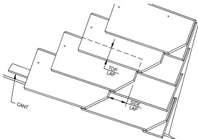
DUTCH LAP SLATE LAYOUT
