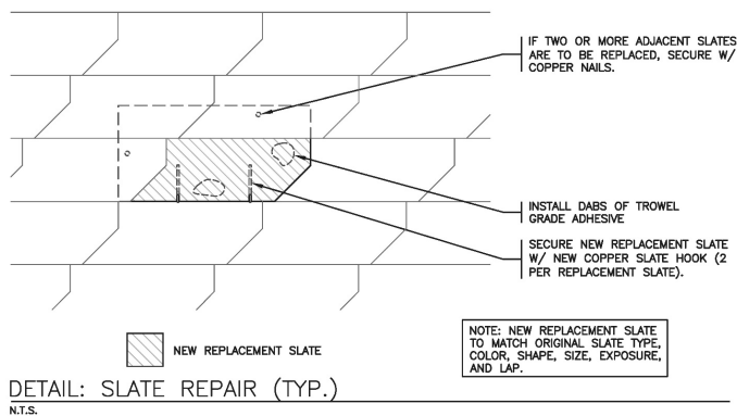
Figure 13: Slate repair in a Dutch Lap roof.
