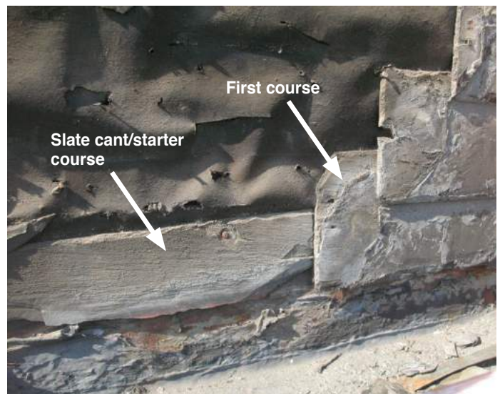
Figure 8: Example of a combination cant and starter slate at the eave of a 142-year old roof.
